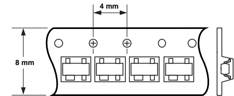
Figure 10. Options -TR1, -TR2 for SOT-143 Packages.
