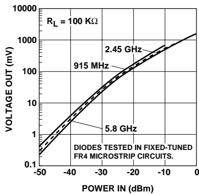
Figure 4. +25°C Output Voltage vs. Input Power, HSMS-2850 at Zero Bias, HSMS-2860 at 3 \mu A Bias.
