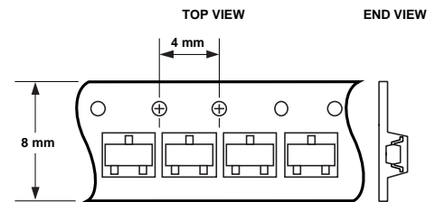
Figure 9. Options -TR1, -TR2 for SOT-23 Packages.
